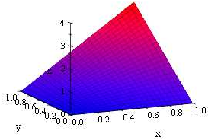
Joint pdf of X and Y for exercise 4.7.9
