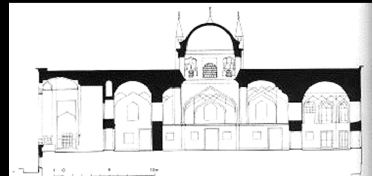
127 Çinili Köşk, Istanbul. Elevation, scale 1 : 250. It has pizzenovsk in the Roman manner.
